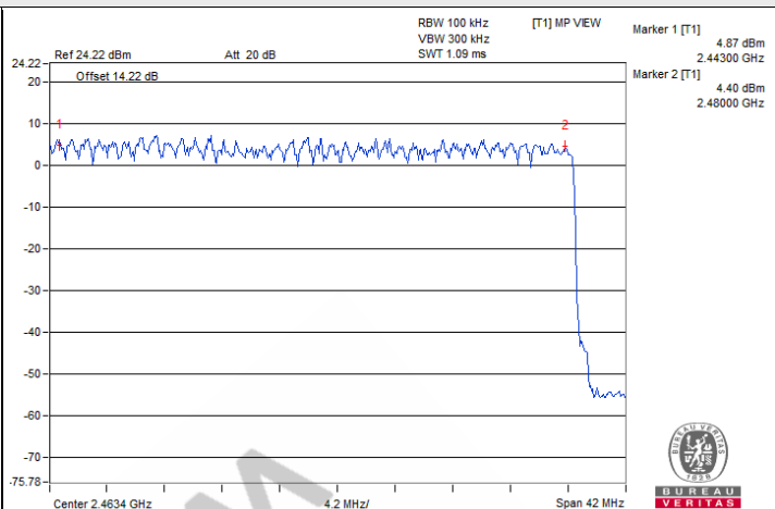
8DPSK 2TX / Chain 0 (Right side)
