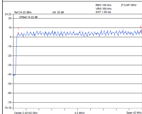
8DPSK 2TX / Chain 0 (Left side)
